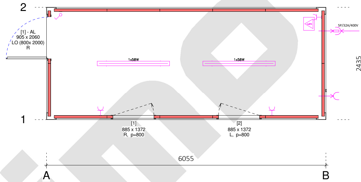
Plan view 1 : 50
