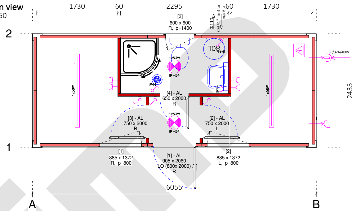
Floor plate
