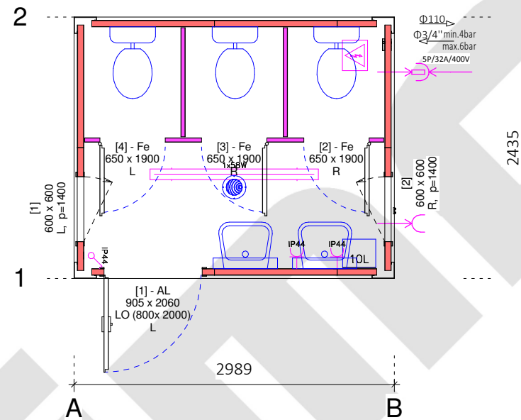
Plan view 1 : 50
