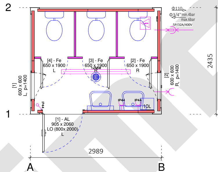
Plan view 1 : 50
